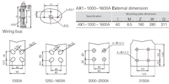
AX1-1000~3150A series lengthways Manual changeover switch boundary and installation dimension
