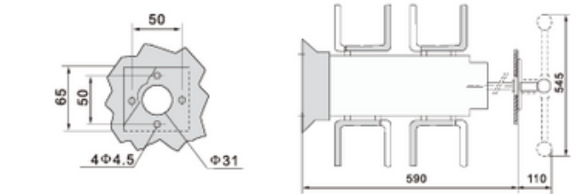
AX1-1000~3150A installation dimension table
