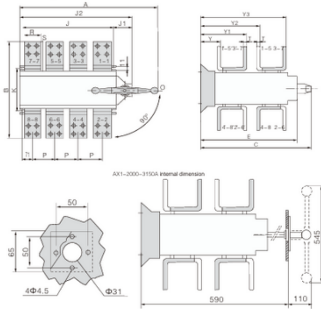
AX1-1000~3150A series lengthways Manual changeover switch boundary and installation dimension
